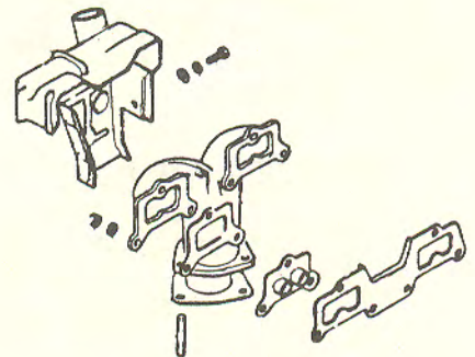
1800 EXHAUST MANIFOLD
