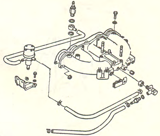
TYPICAL 4 CYLINDER INTAKE MANIFOLD
