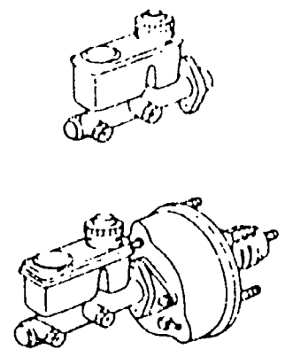
TANDEM MASTER CYL. & VACUUM POWER ASSIST SYSTEM
