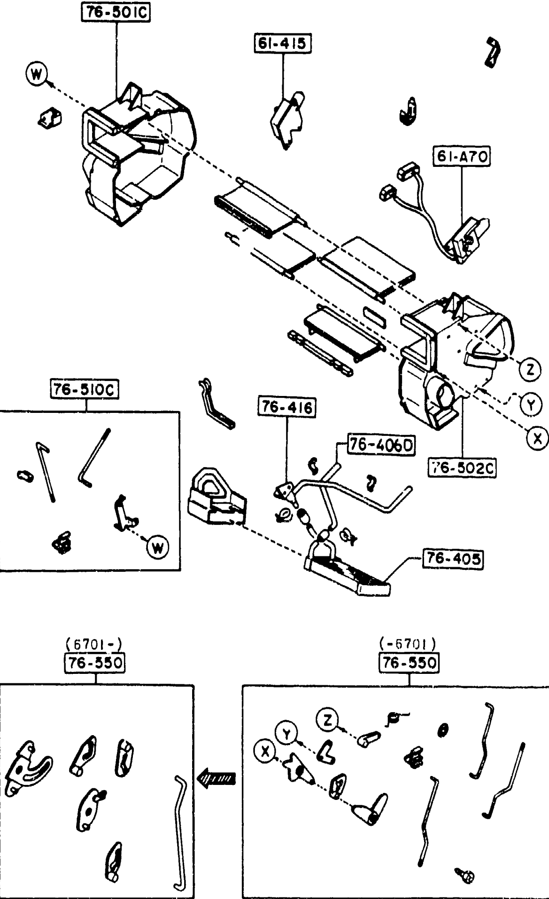
COMPONENTS OF FB01-61-130A
