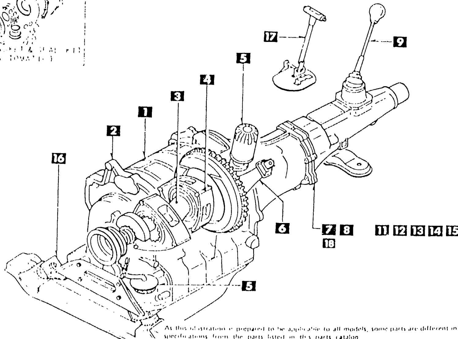
TRANSMISSION CASE (MANUAL)
